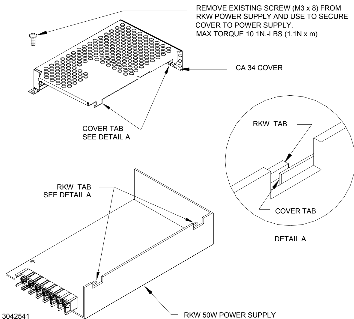
FIGURE 1. CA 34-R COVER INSTALLATION
